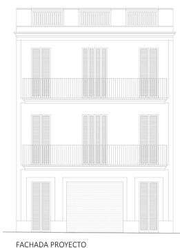
Façade project (3 floors)
