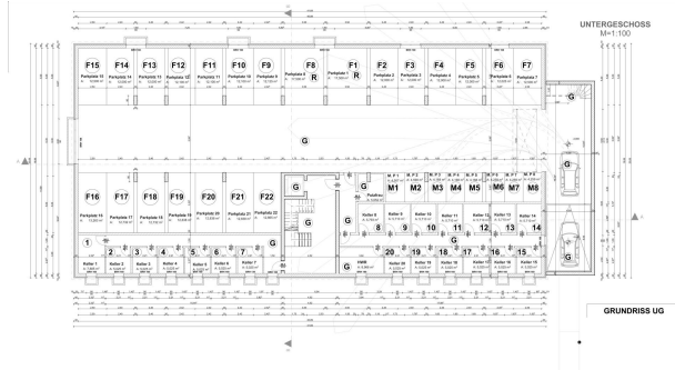
Grundriss_UG
